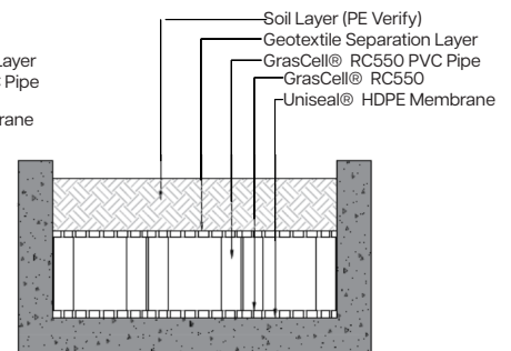
GrasCell® RC550 VOID FILLER TYPICAL DETAIL
