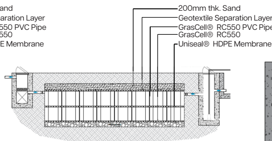
GrasCell® RC550 RETENTION TANK TYPICAL DETAIL
