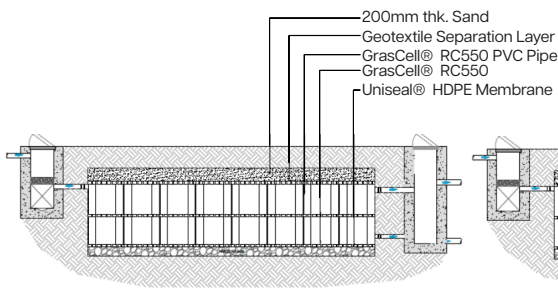
GrasCell® RC550 DETENTION TANK TYPICAL DETAIL
